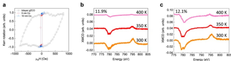
Fig. 3: Room-temperature ferromagnetism in 2D gZCO.
